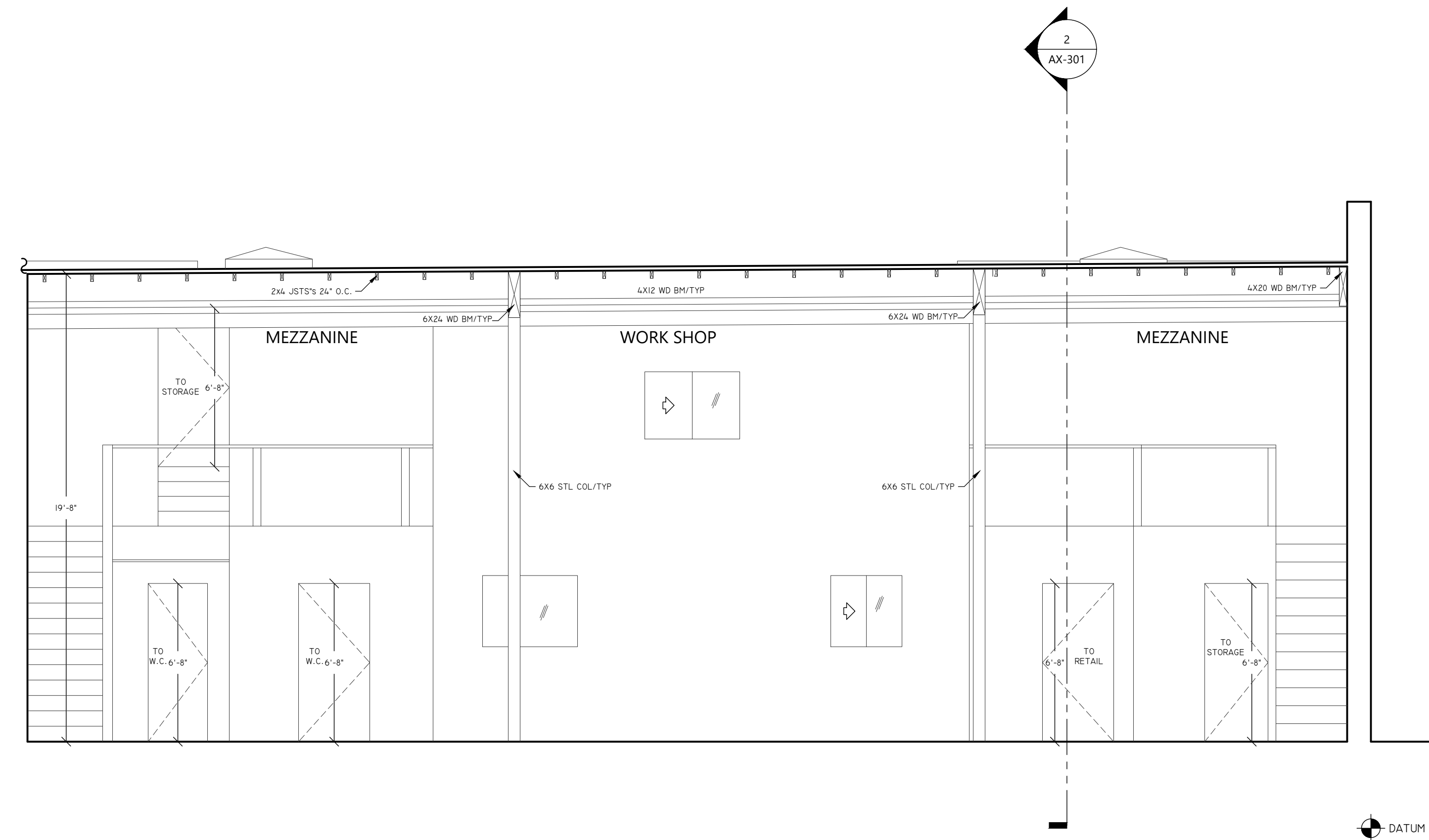
1 EXISTING CROSS SECTION
